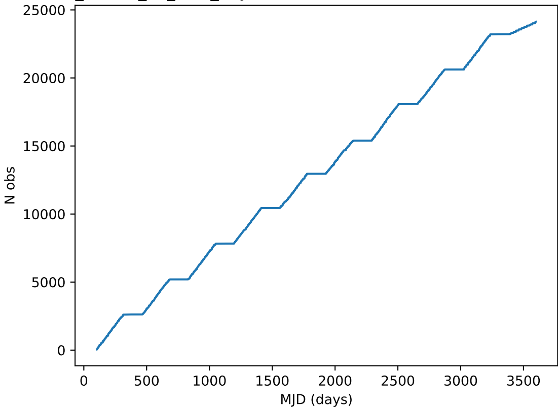
ddf_loaded_fl8_v3.4_10yrs all bands: DD:EDFS Cumulative NVisits
