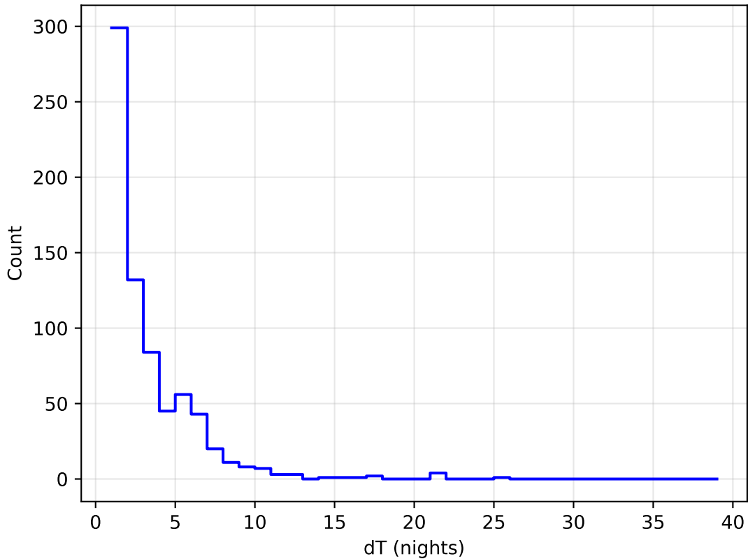
ddf_loaded_fl8_v3.4_10yrs all bands: DD:ECDFS Delta Nights Histogram
