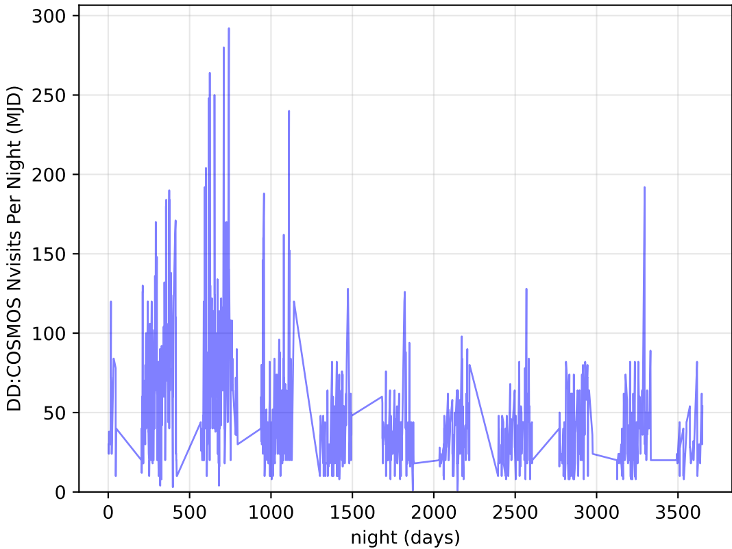
ddf_loaded_fl8_v3.4_10yrs all bands: DD: COSMOS Nvisits Per Night
