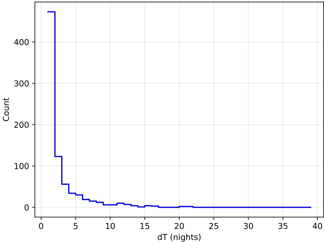
ddf_loaded_fl8_v3.4_10yrs all bands: DD: COSMOS Delta Nights Histogram
