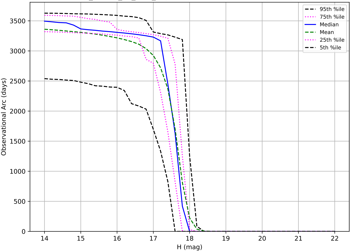
ddf_loaded_fl4_v3.4_10yrs: Observational Arc Length Trojan
