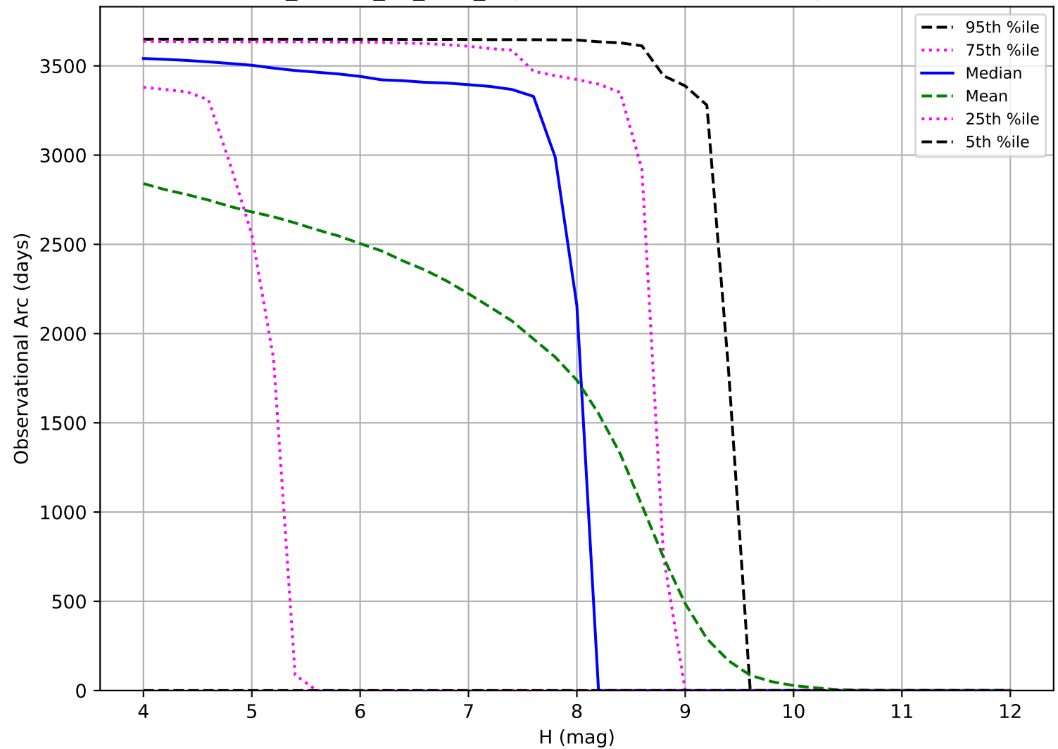
ddf_loaded_fl4_v3.4_10yrs: Observational Arc Length TNO
