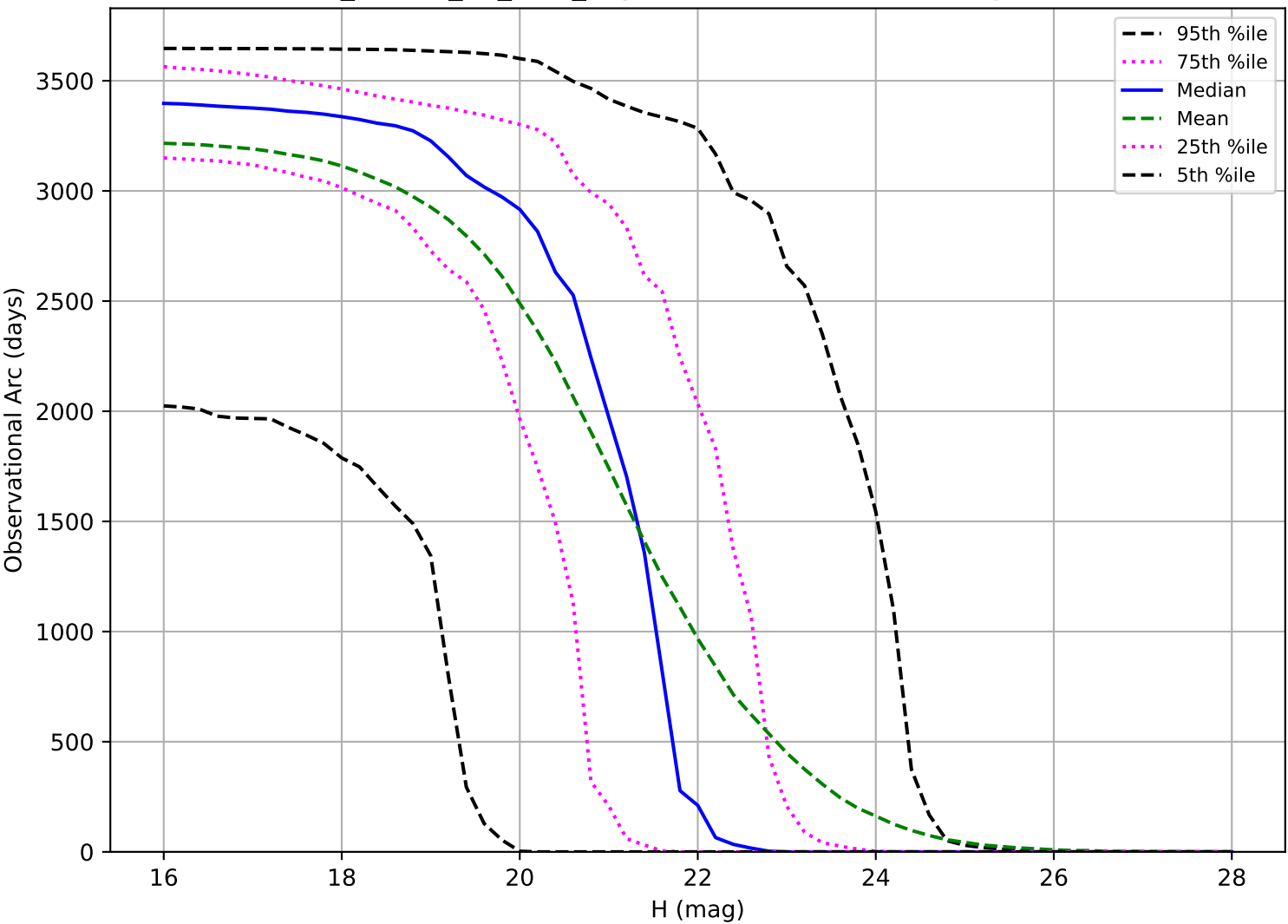
ddf_loaded_fl4_v3.4_10yrs: Observational Arc Length PHA
