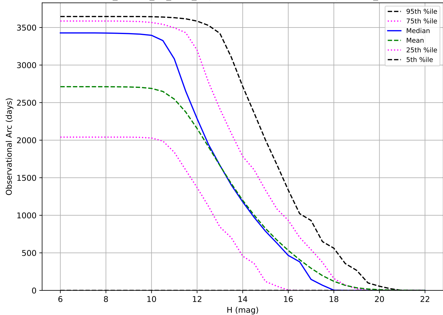
ddf_loaded_fl4_v3.4_10yrs: Observational Arc Length OCC_r5
