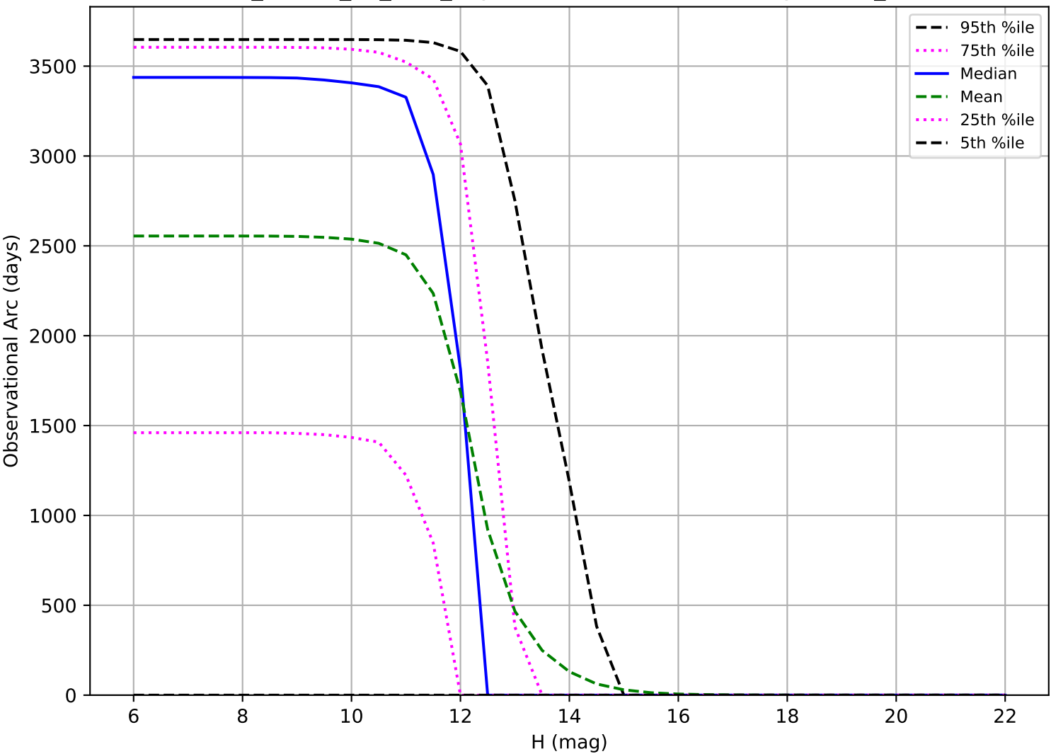
ddf_loaded_fl4_v3.4_10yrs: Observational Arc Length OCC_r20
