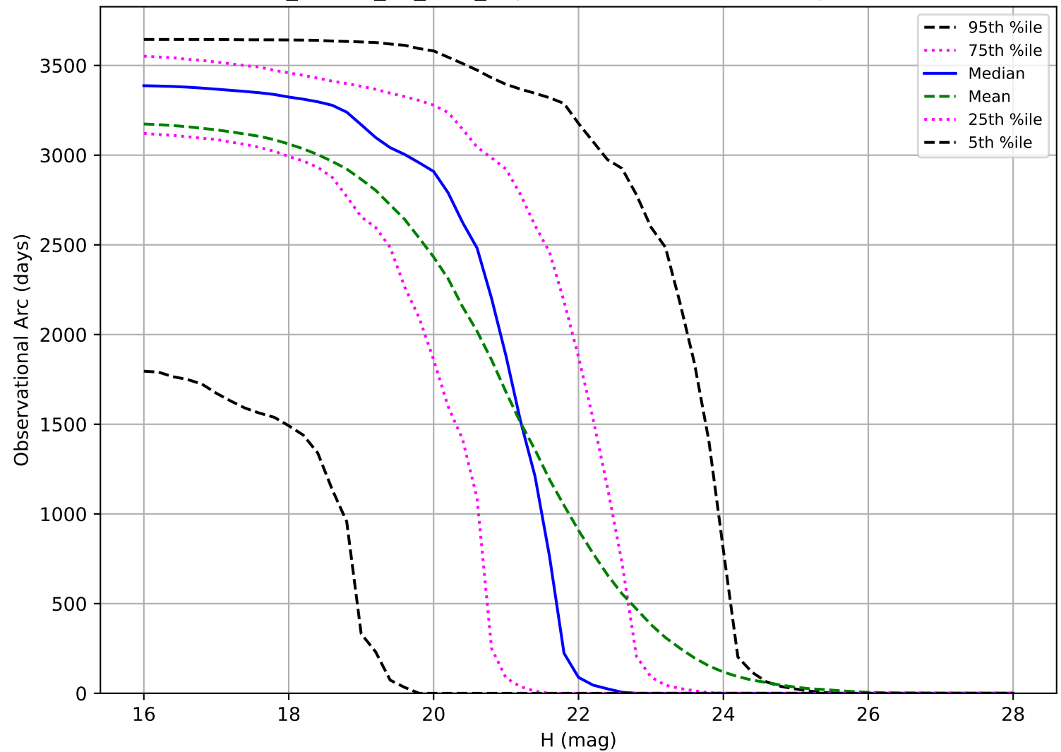
ddf_loaded_fl4_v3.4_10yrs: Observational Arc Length NEO
