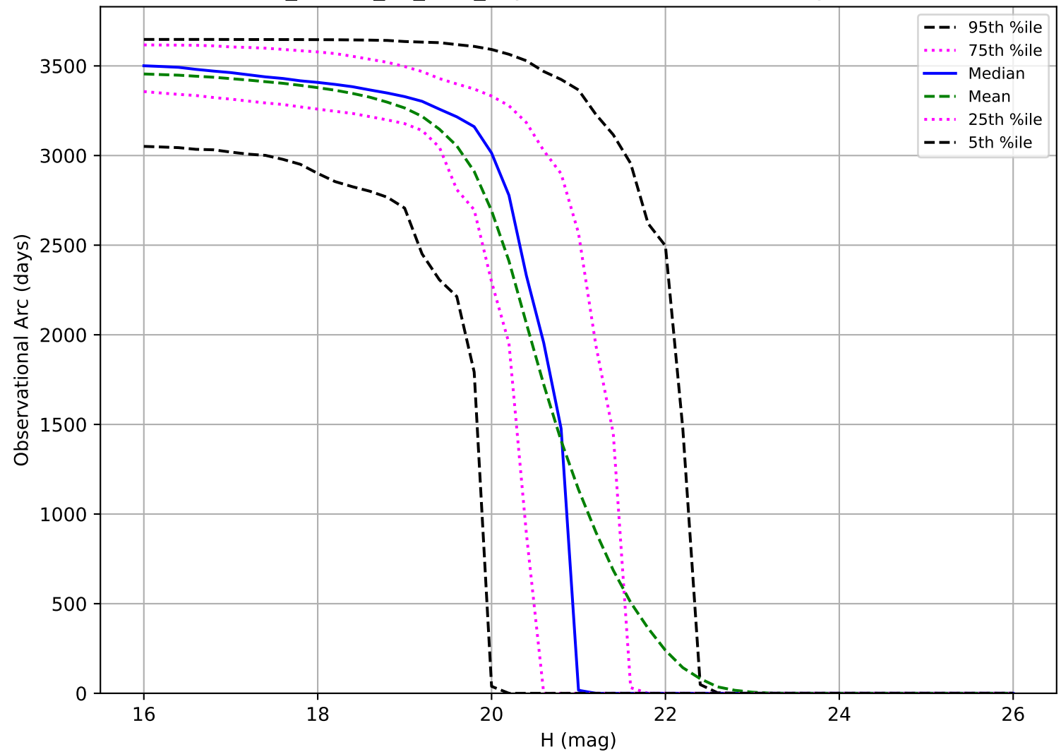
ddf_loaded_fl4_v3.4_10yrs: Observational Arc Length MBA
