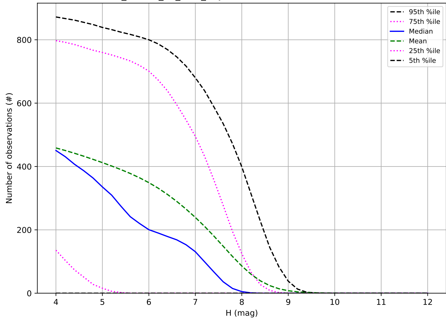
ddf_loaded_fl4_v3.4_10yrs: Number of observations TNO
