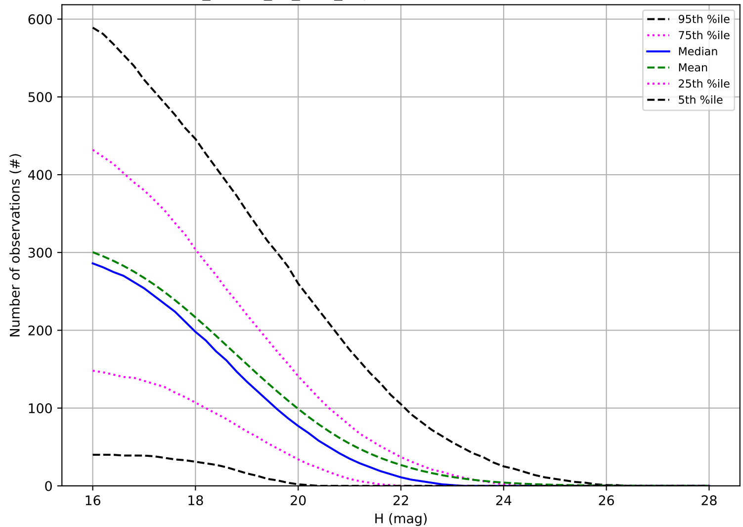
ddf_loaded_fl4_v3.4_10yrs: Number of observations PHA
