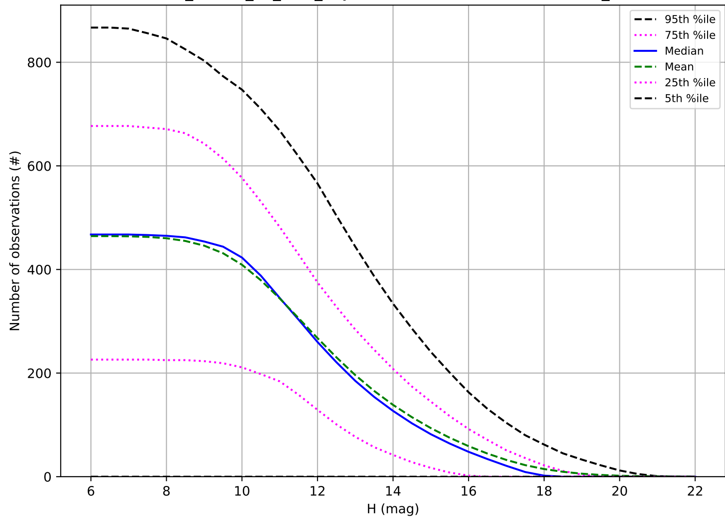
ddf_loaded_fl4_v3.4_10yrs: Number of observations OCC_r5
