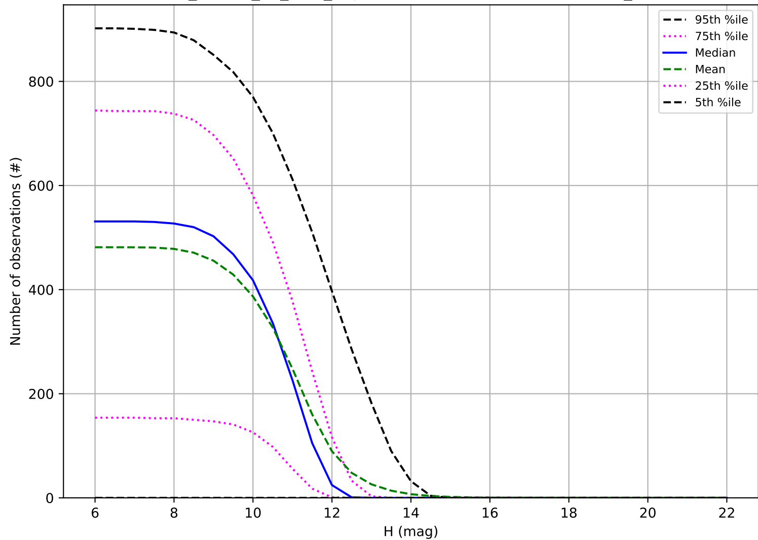
ddf_loaded_fl4_v3.4_10yrs: Number of observations OCC_r20
