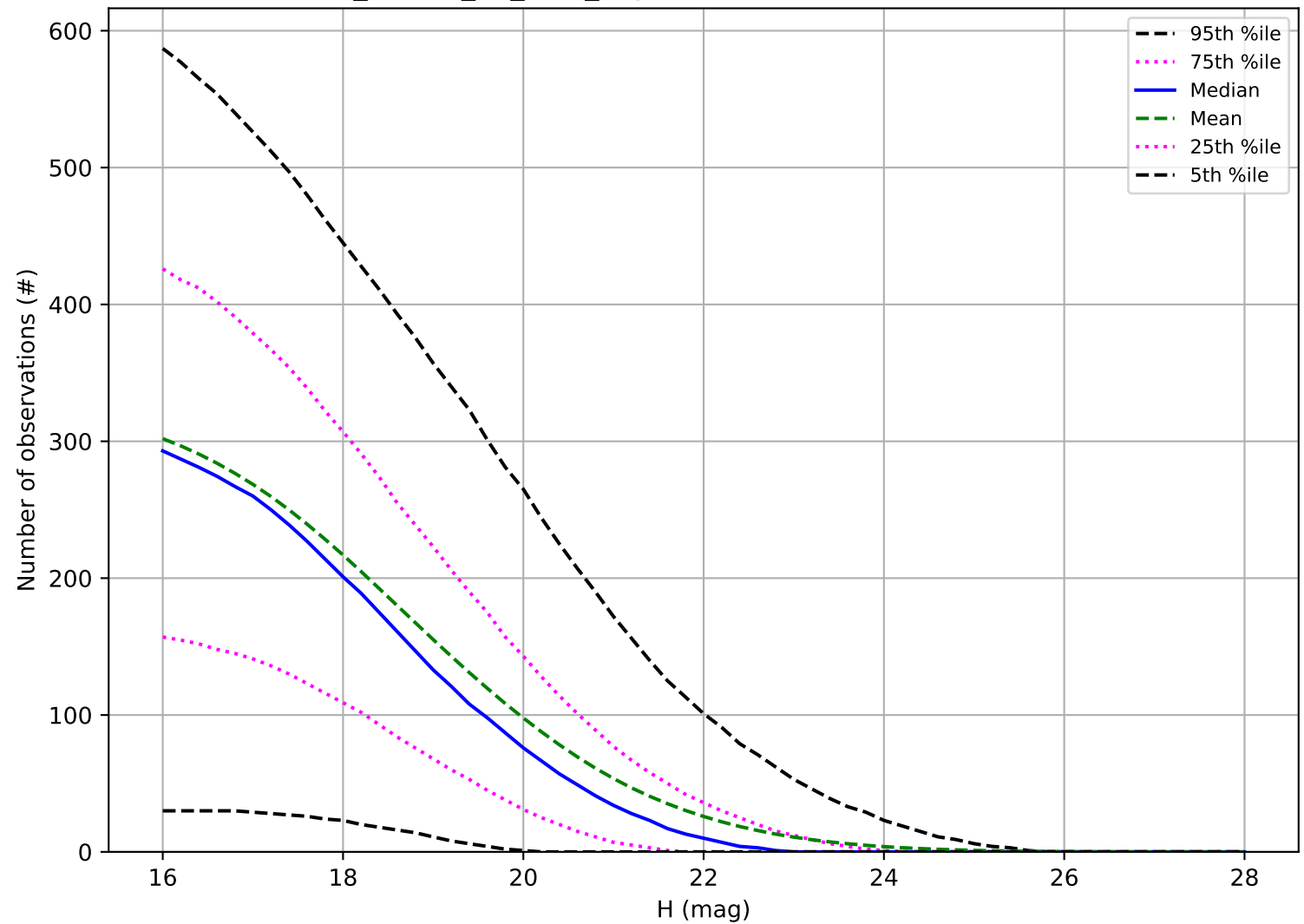
ddf_loaded_fl4_v3.4_10yrs: Number of observations NEO
