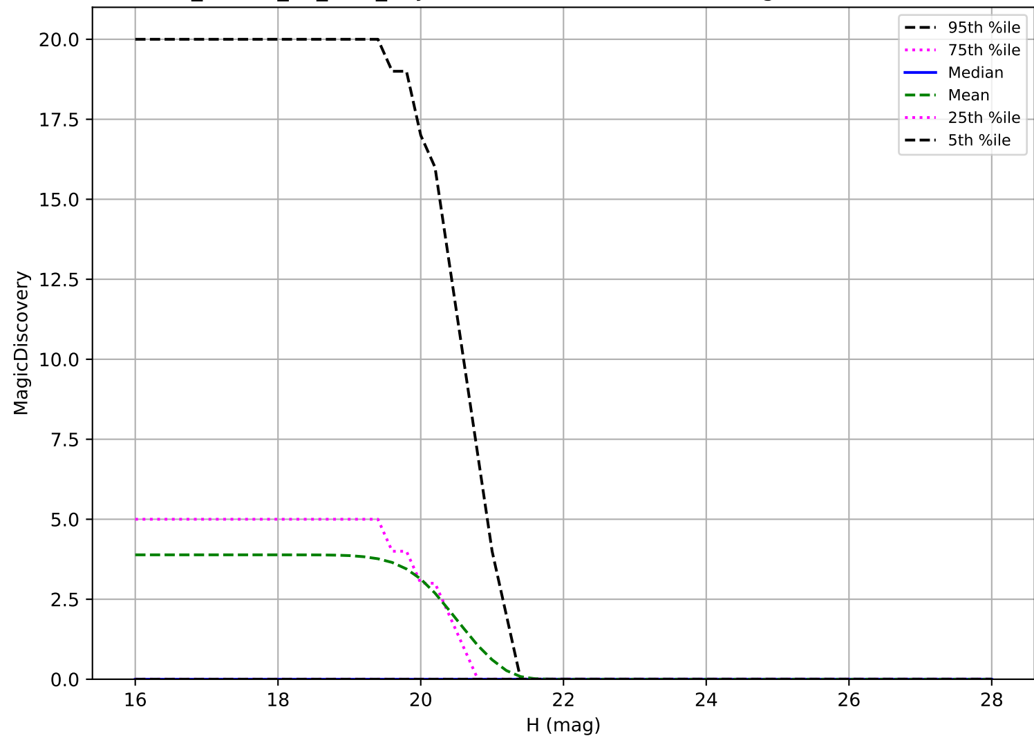
ddf_loaded_fl4_v3.4_10yrs: Vatira 6 detections in 60 nights detection loss
