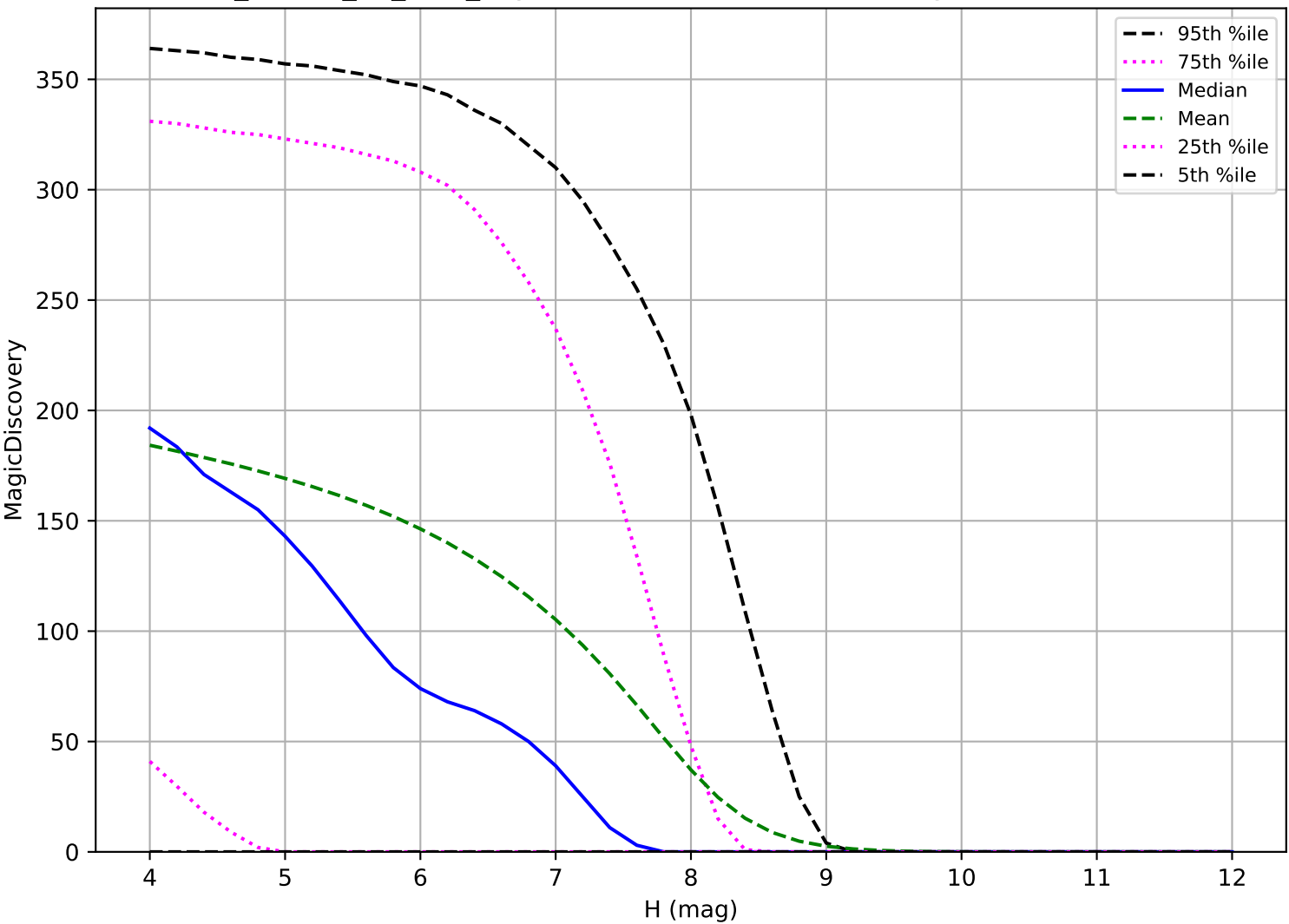
ddf_loaded_fl4_v3.4_10yrs: TNO 6 detections in 60 nights detection loss
