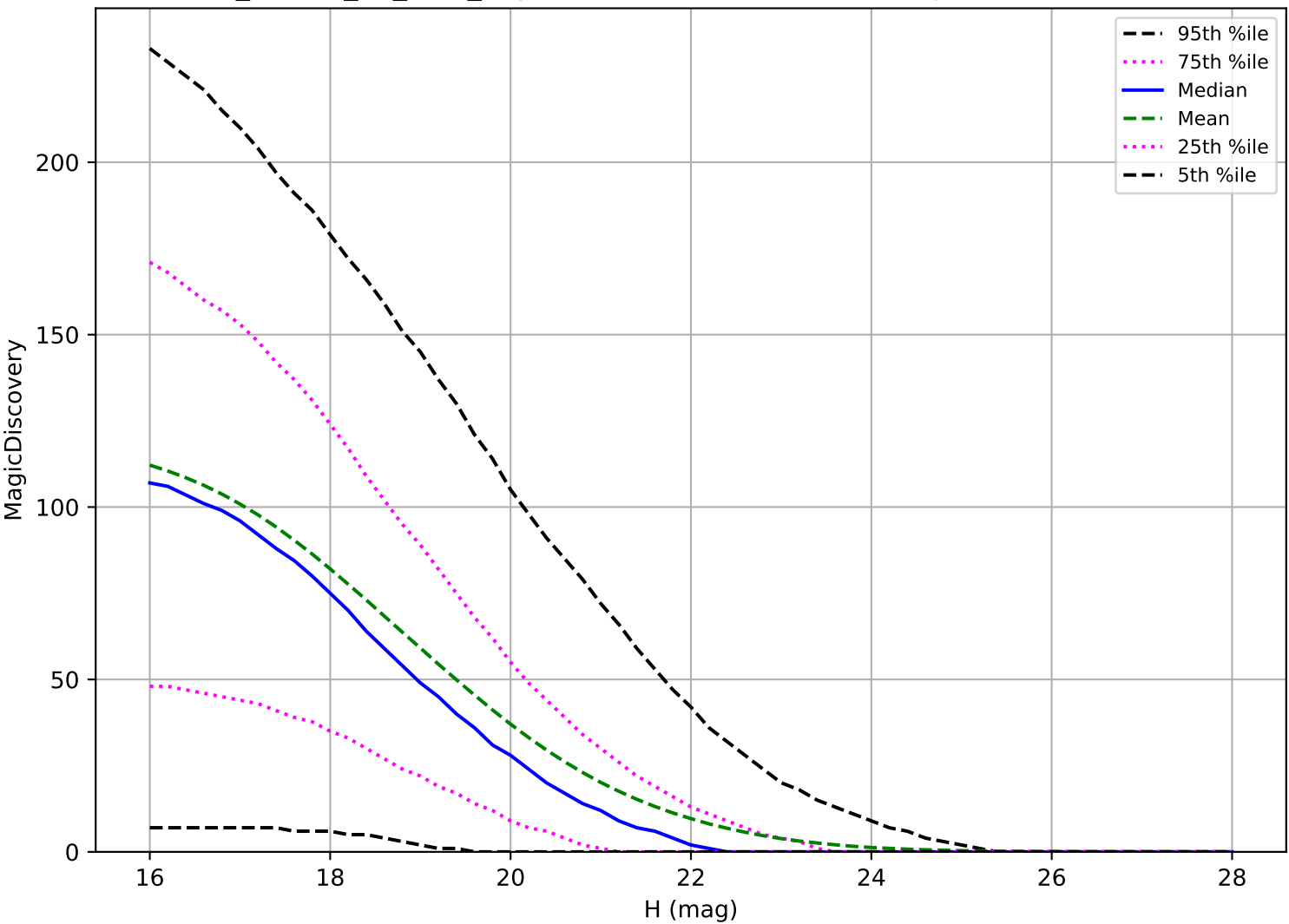
ddf_loaded_fl4_v3.4_10yrs: PHA 6 detections in 60 nights detection loss
