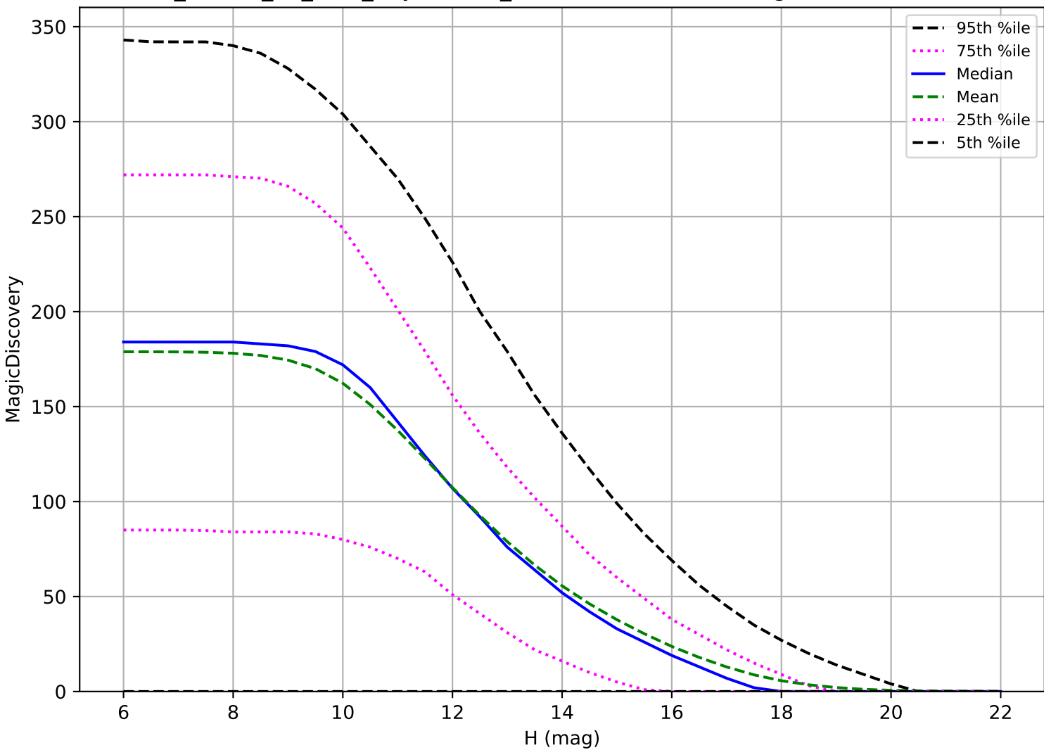
ddf_loaded_fl4_v3.4_10yrs: OCC_r5 6 detections in 60 nights detection loss
