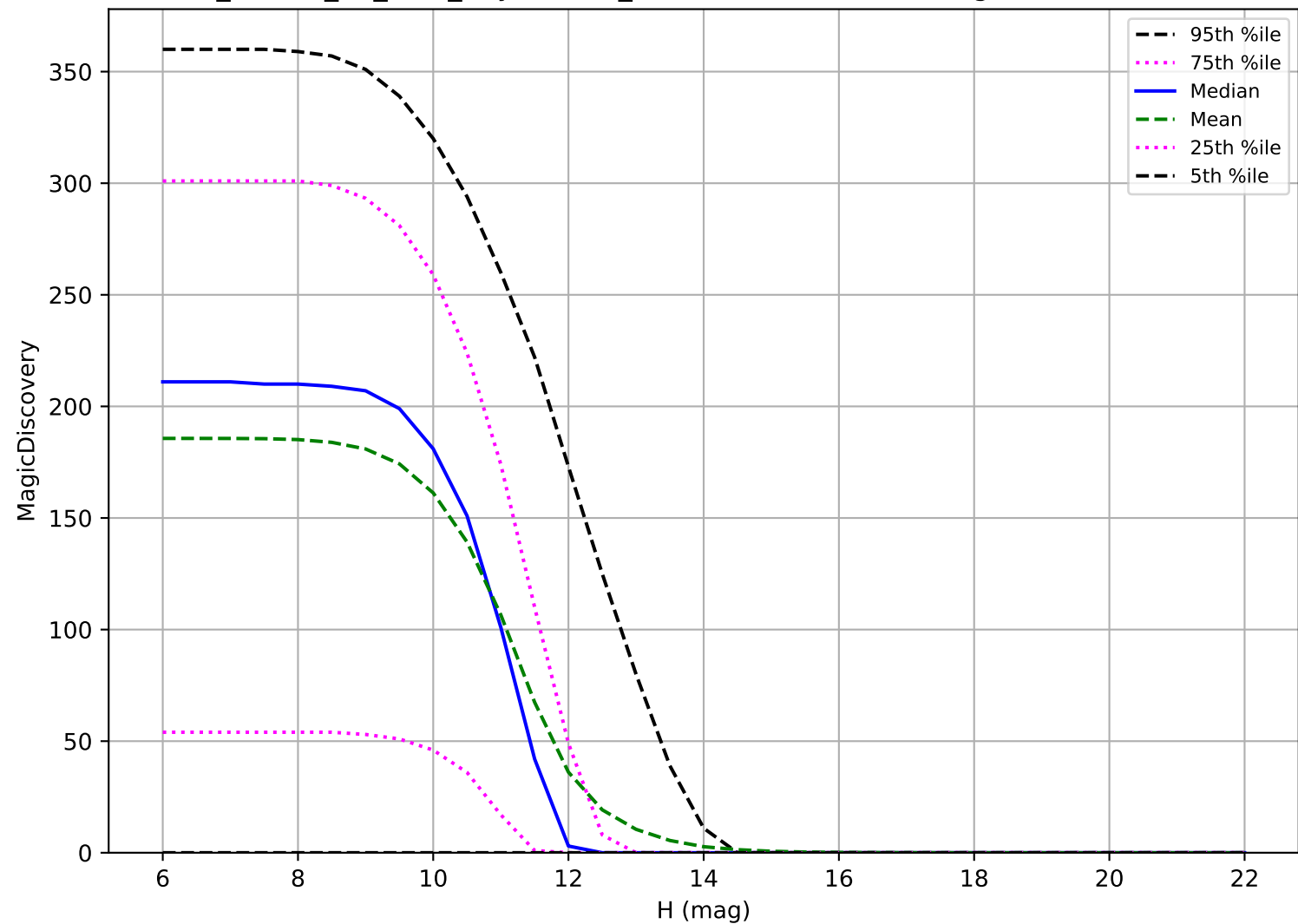
ddf_loaded_fl4_v3.4_10yrs: OCC_r20 6 detections in 60 nights detection loss
