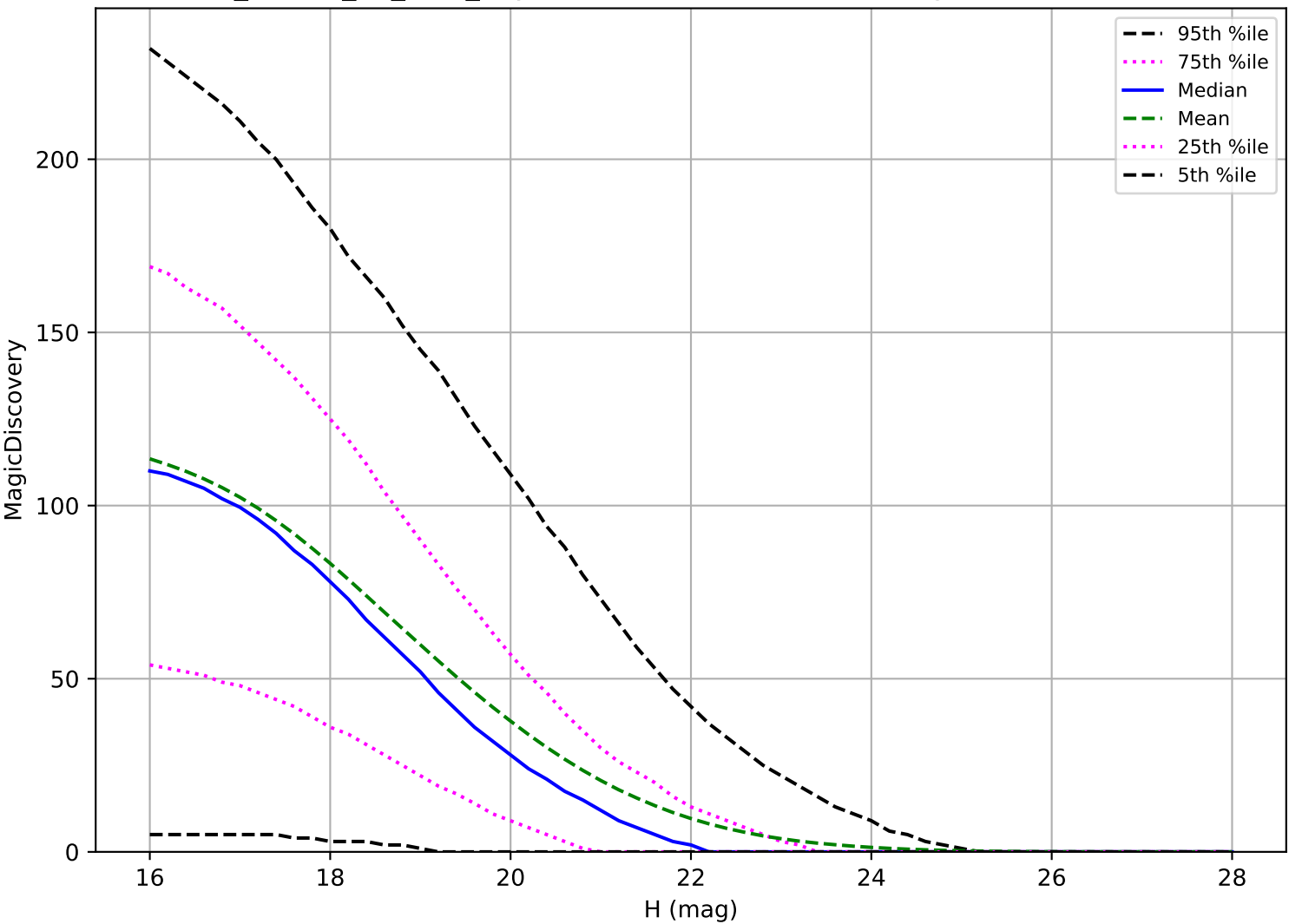
ddf_loaded_f14_v3.4_10yrs: NEO 6 detections in 60 nights detection loss
