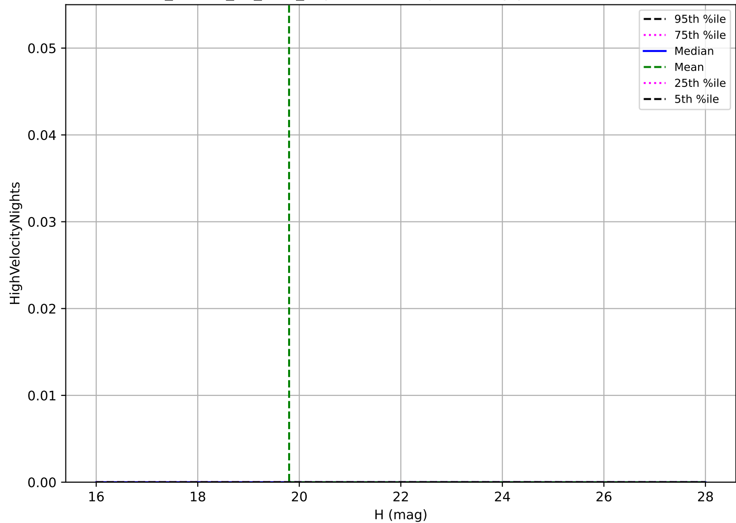
ddf_loaded_fl4_v3.4_10yrs: Vatira High velocity pair detection loss
