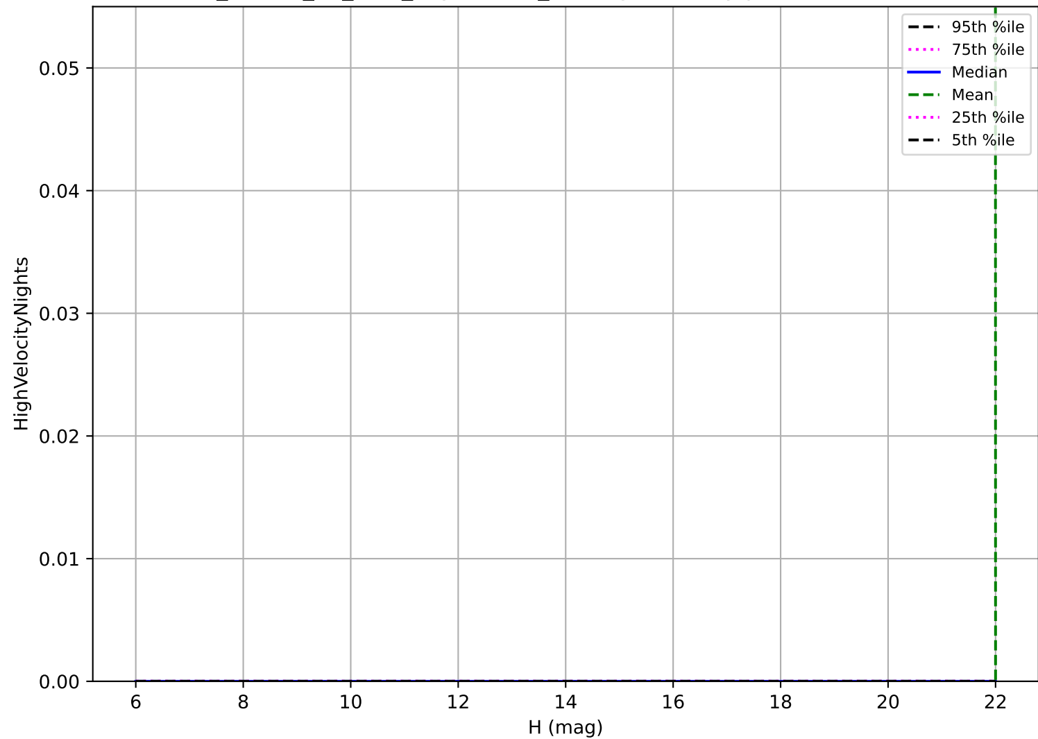
ddf_loaded_fl4_v3.4_10yrs: OCC_r20 High velocity pair detection loss
