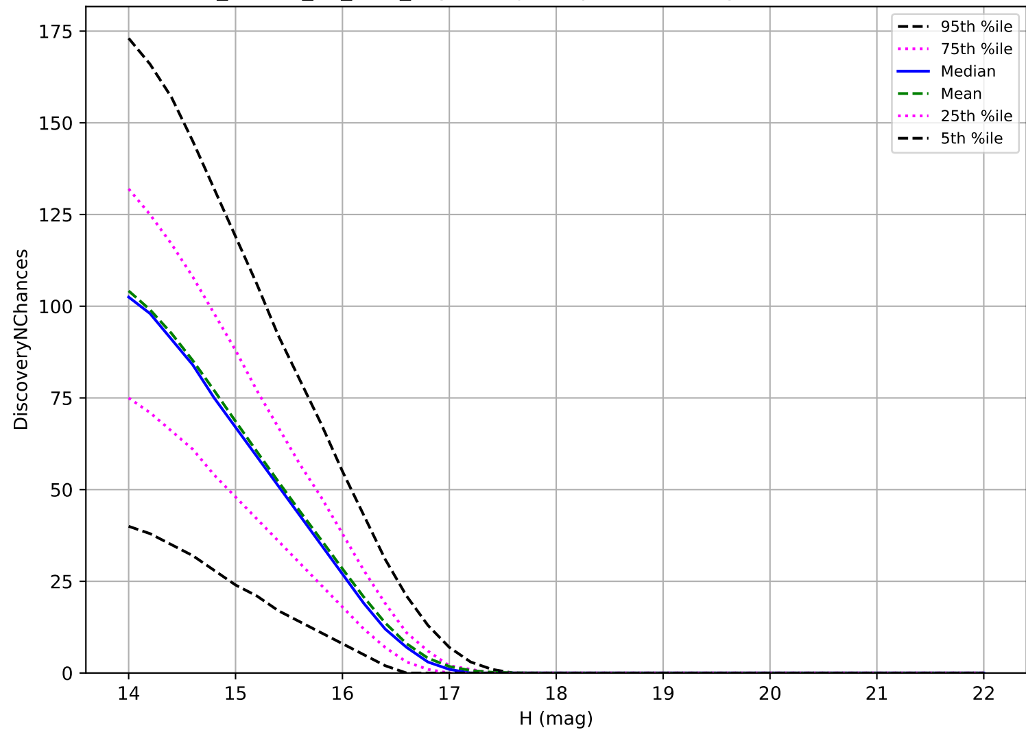
ddf_loaded_f14_v3.4_10yrs: Trojan 3 pairs in 15 nights detection loss
