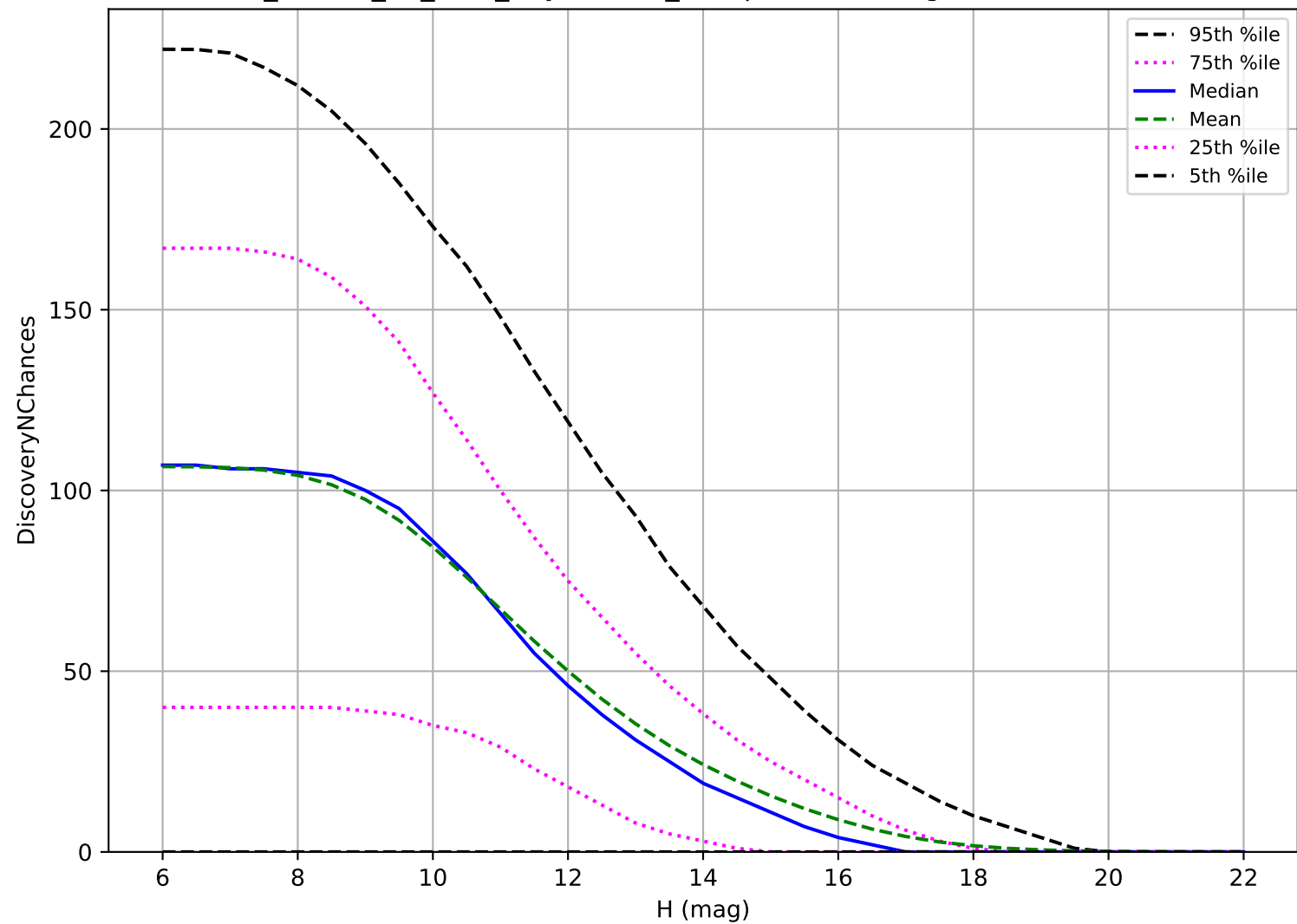
ddf_loaded_fl4_v3.4_10yrs: OCC_r5 3 pairs in 15 nights detection loss
