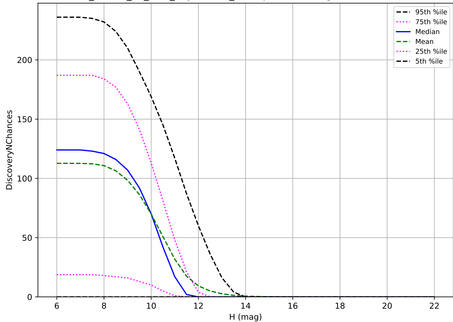
ddf_loaded_fl4_v3.4_10yrs: OCC_r20 3 pairs in 15 nights detection loss
