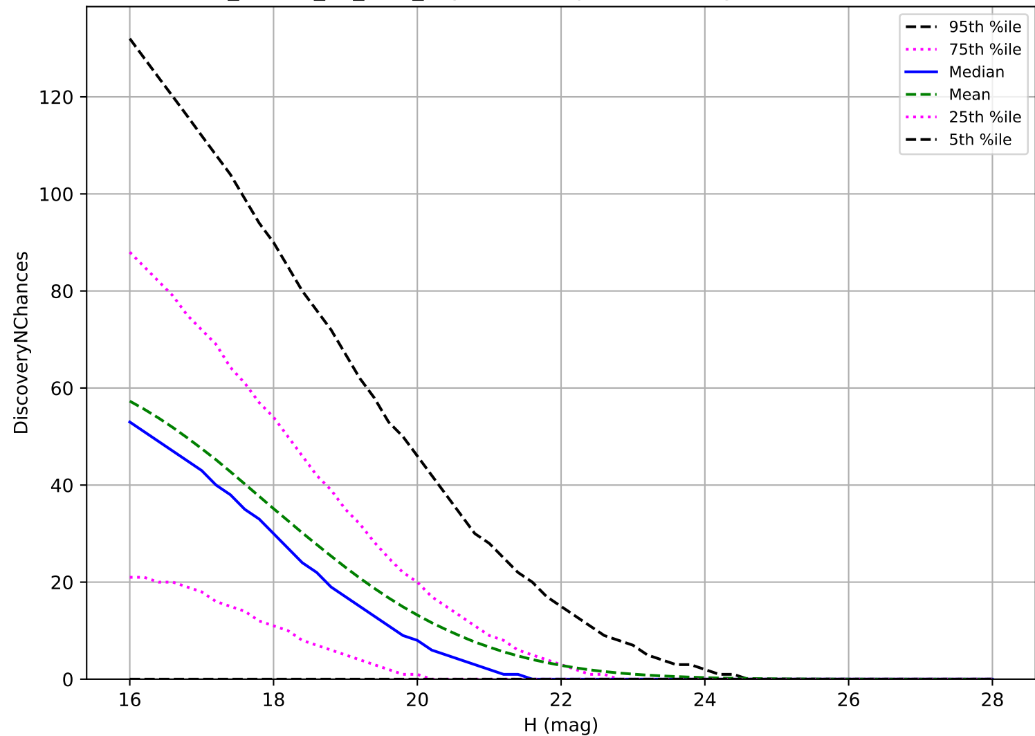
ddf_loaded_fl4_v3.4_10yrs: NEO 3 pairs in 15 nights detection loss
