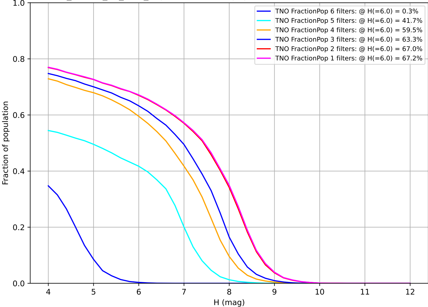
ddf_loaded_fl4_v3.4_10yrs: Fraction of population with colors in X filters TNO
