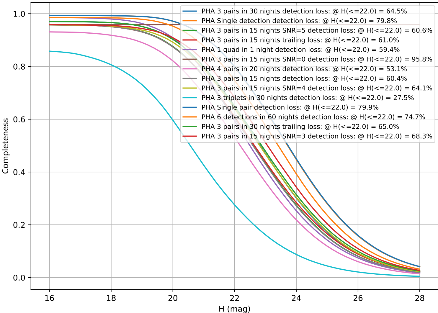
ddf_loaded_fl4_v3.4_10yrs: CumulativeCompleteness
