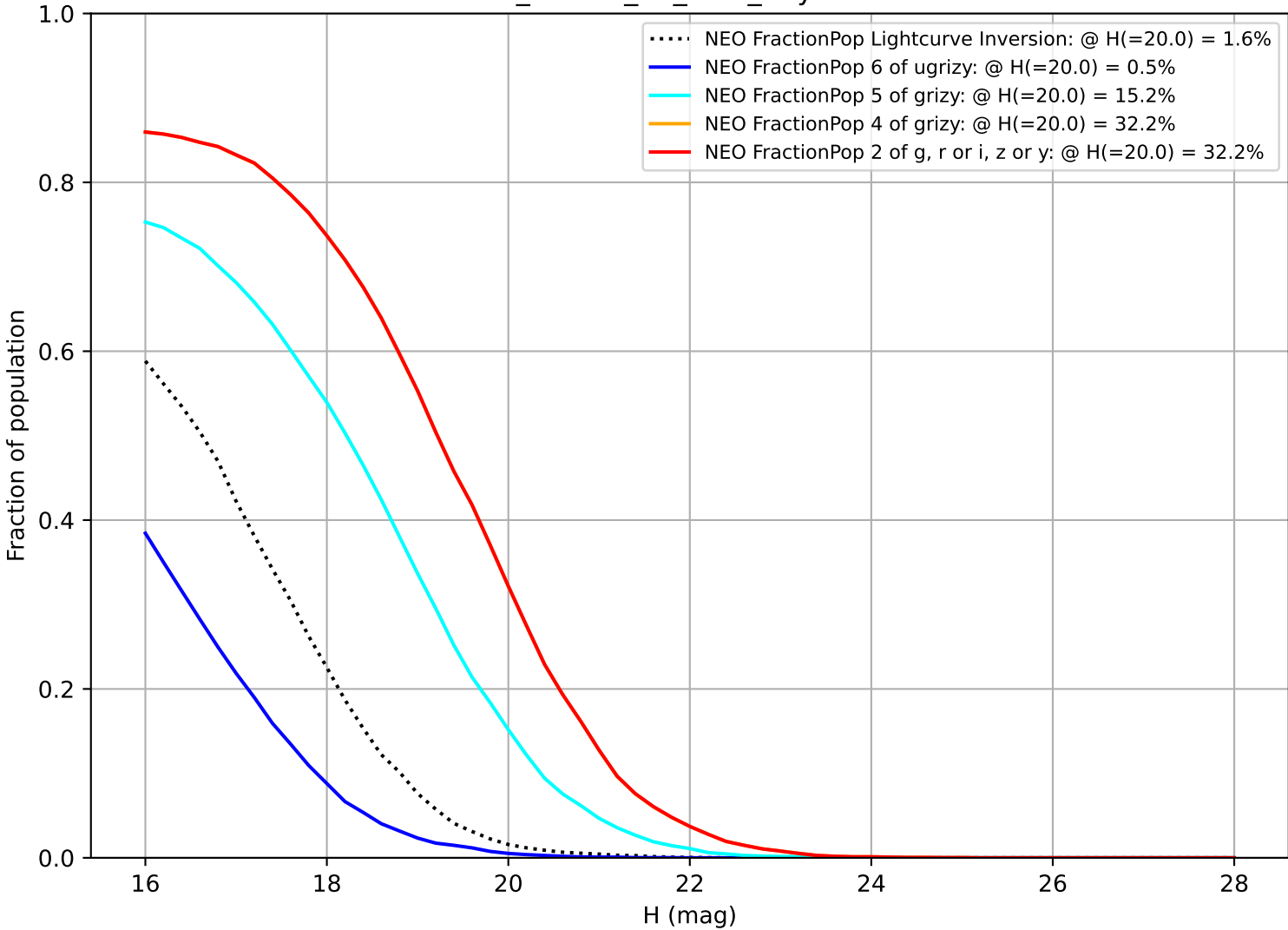
ddf_loaded_fl4_v3.4_10yrs NEO
