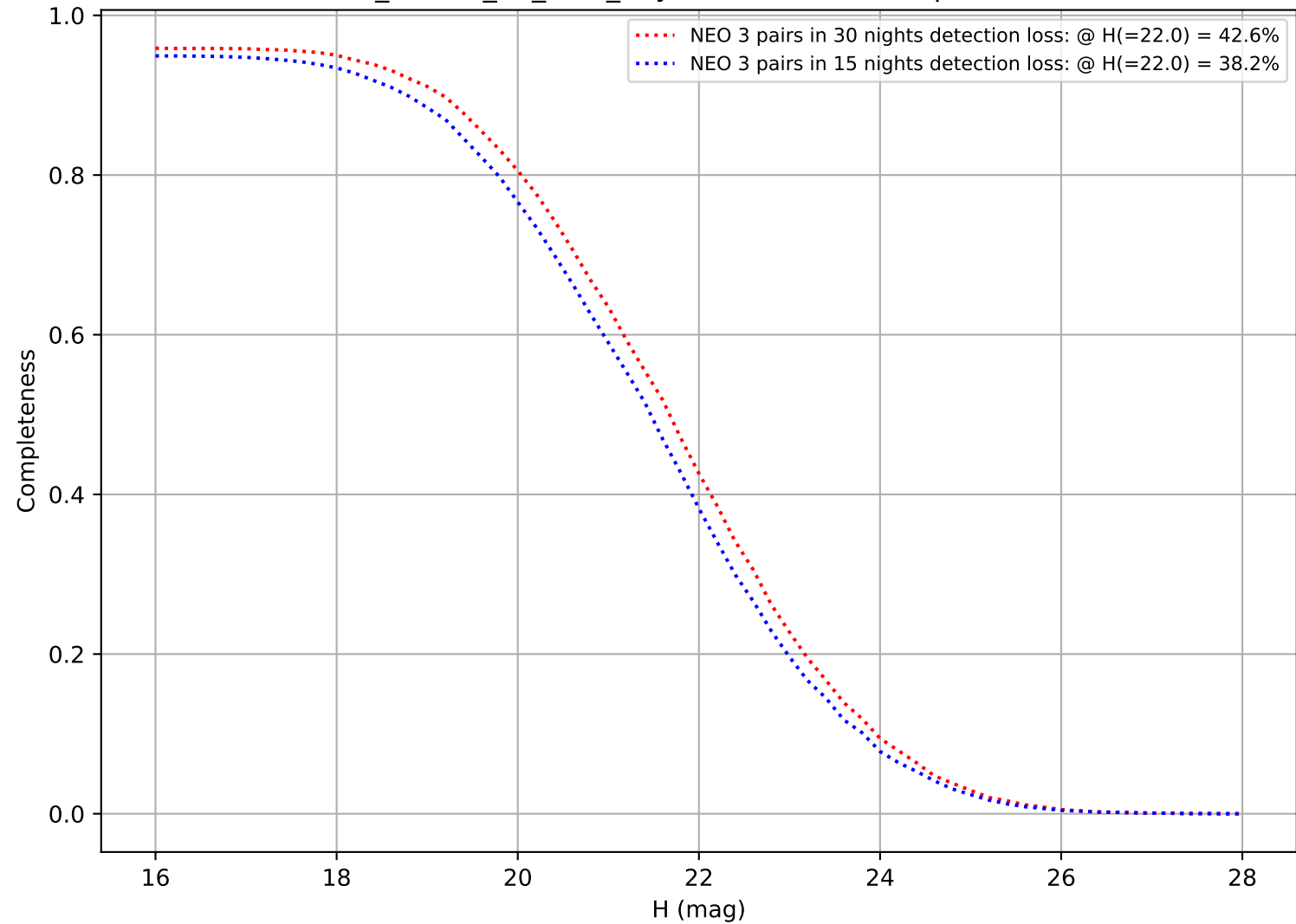
ddf_loaded_fl4_v3.4_10yrs: DifferentialCompleteness
