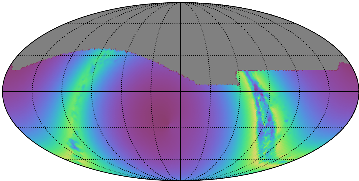
ddf_loaded_fl4_v3.4_10yrs : young_stars
