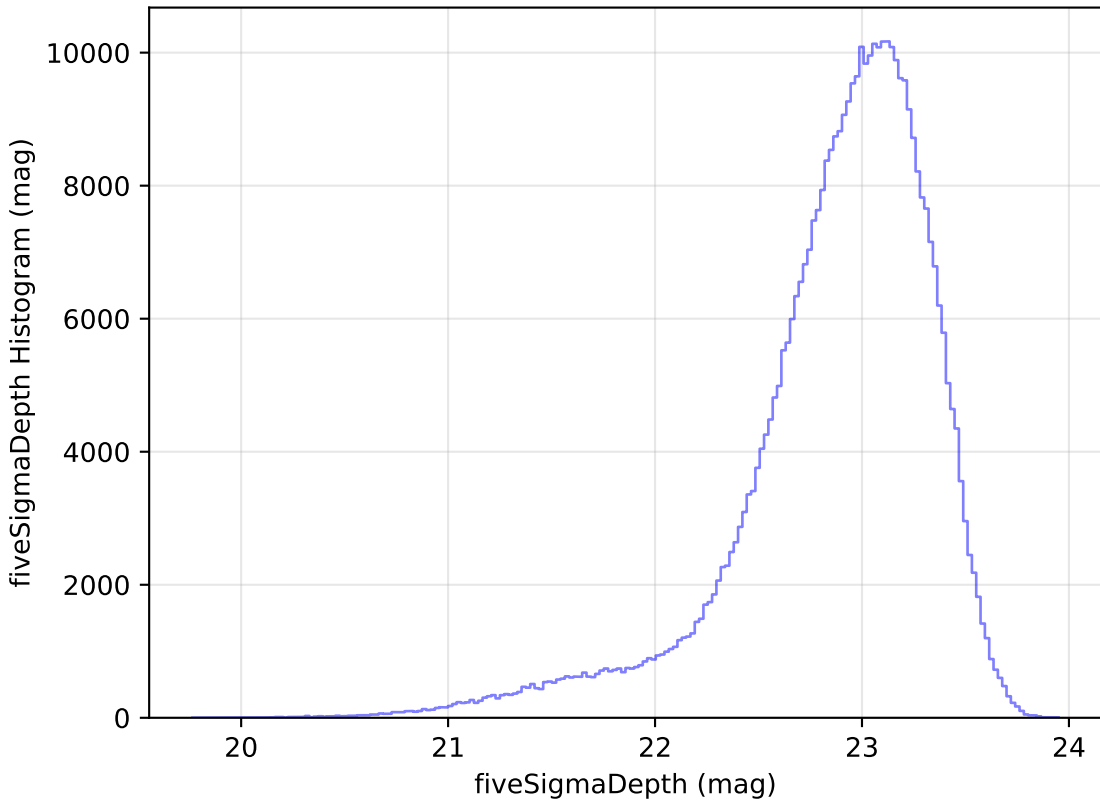
ddf_loaded_fl4_v3.4_10yrs z: fiveSigmaDepth Histogram
