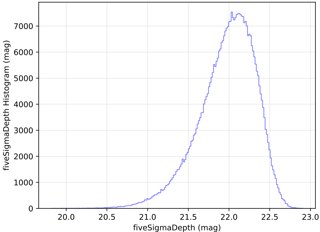
ddf_loaded_fl4_v3.4_10yrs y: fiveSigmaDepth Histogram
