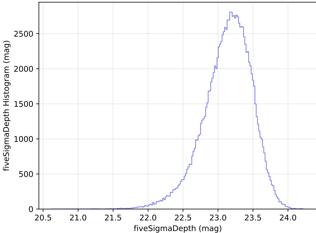
ddf_loaded_fl4_v3.4_10yrs u: fiveSigmaDepth Histogram
