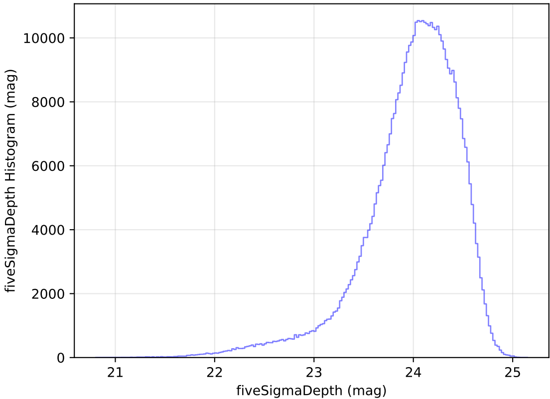
ddf_loaded_fl4_v3.4_10yrs r: fiveSigmaDepth Histogram
