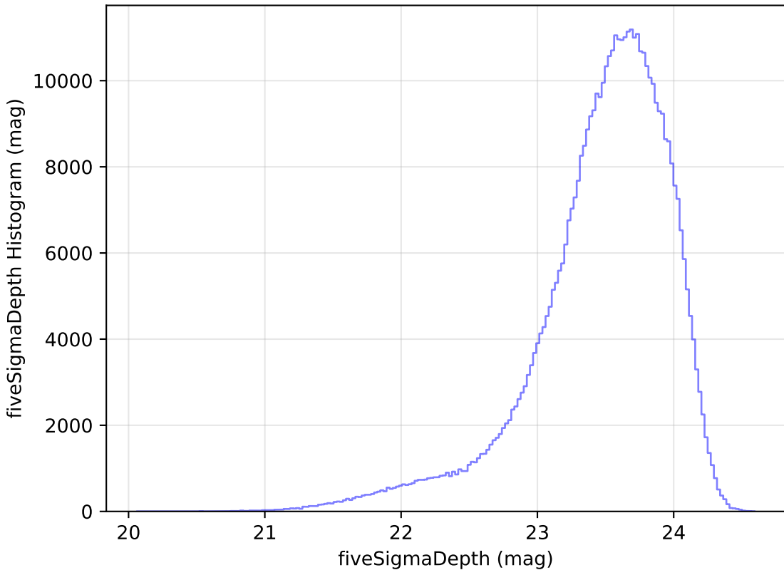
ddf_loaded_fl4_v3.4_10yrs i: fiveSigmaDepth Histogram
