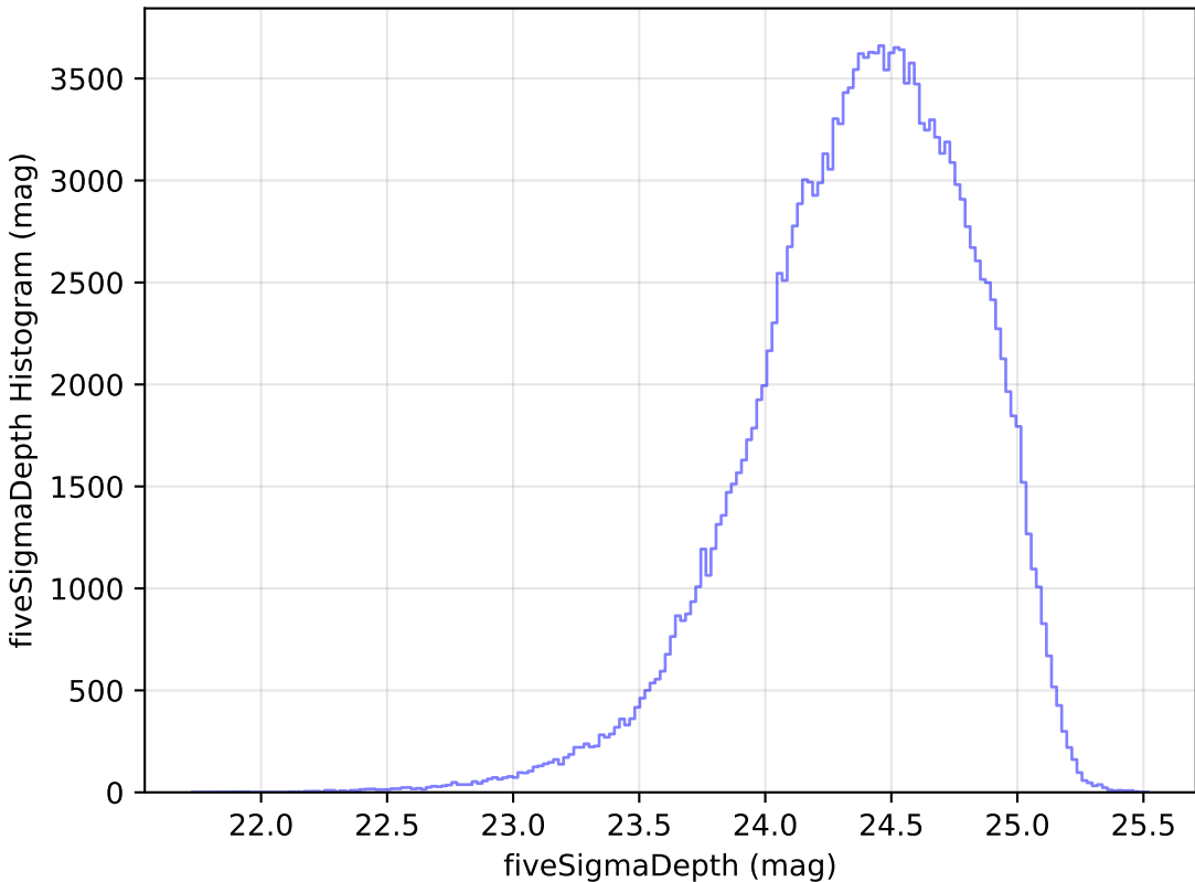
ddf_loaded_fl4_v3.4_10yrs g: fiveSigmaDepth Histogram
