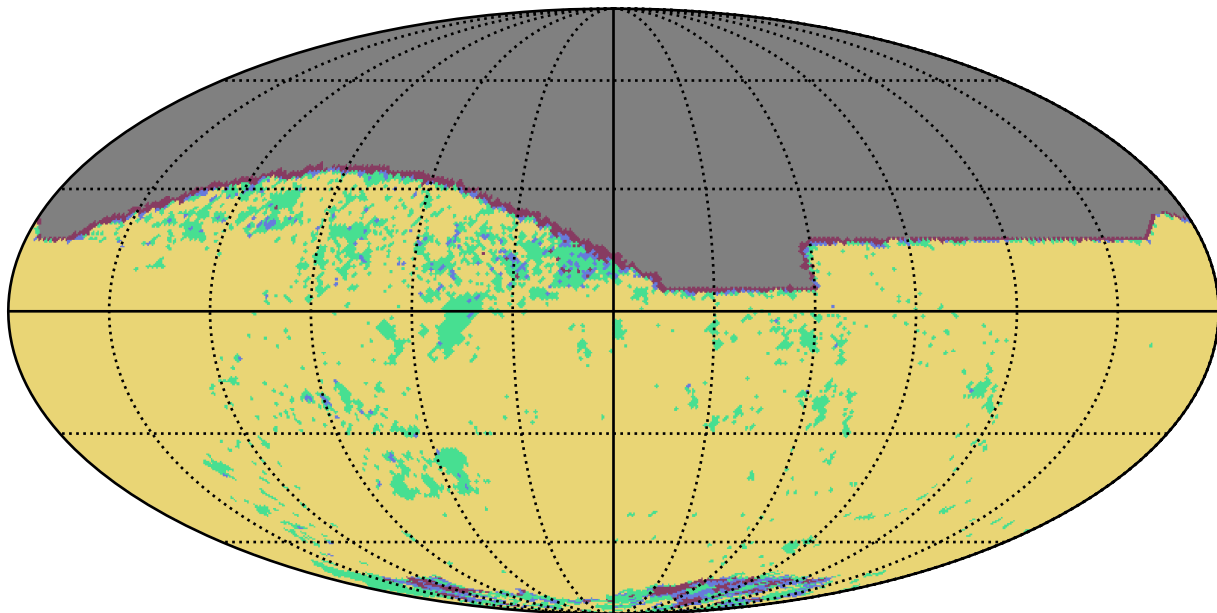
ddf_loaded_fl4_v3.4_10yrs z band: YearCoverage night
