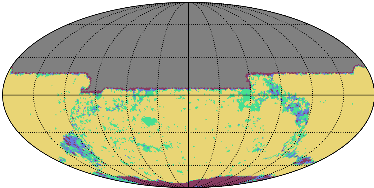
ddf_loaded_fl4_v3.4_10yrs y band: YearCoverage night
