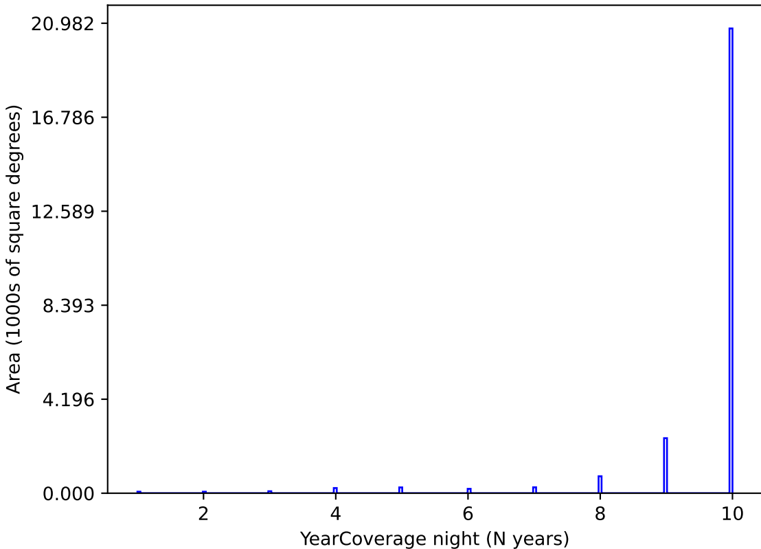
ddf_loaded_fl4_v3.4_10yrs y band: YearCoverage night
