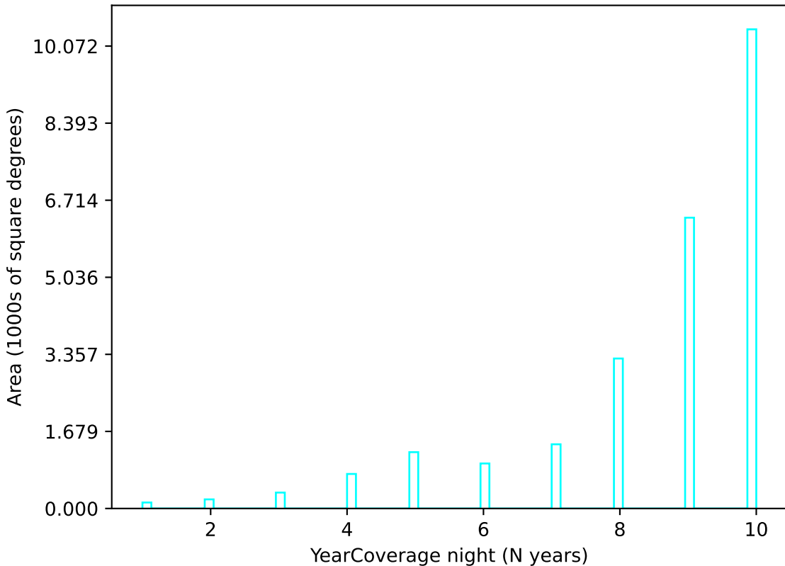
ddf_loaded_fl4_v3.4_10yrs u band: YearCoverage night
