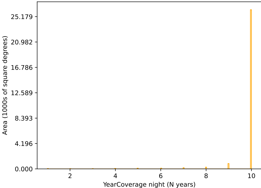
ddf_loaded_fl4_v3.4_10yrs r band: YearCoverage night
