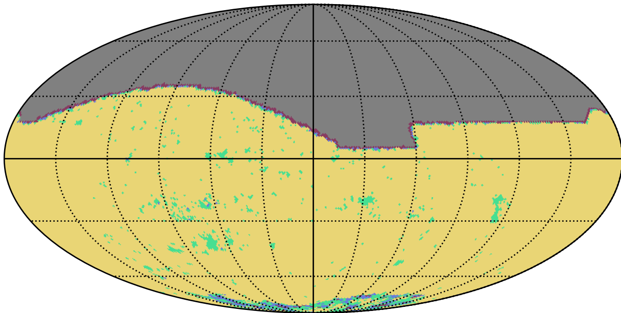
ddf_loaded_fl4_v3.4_10yrs i band: YearCoverage night
