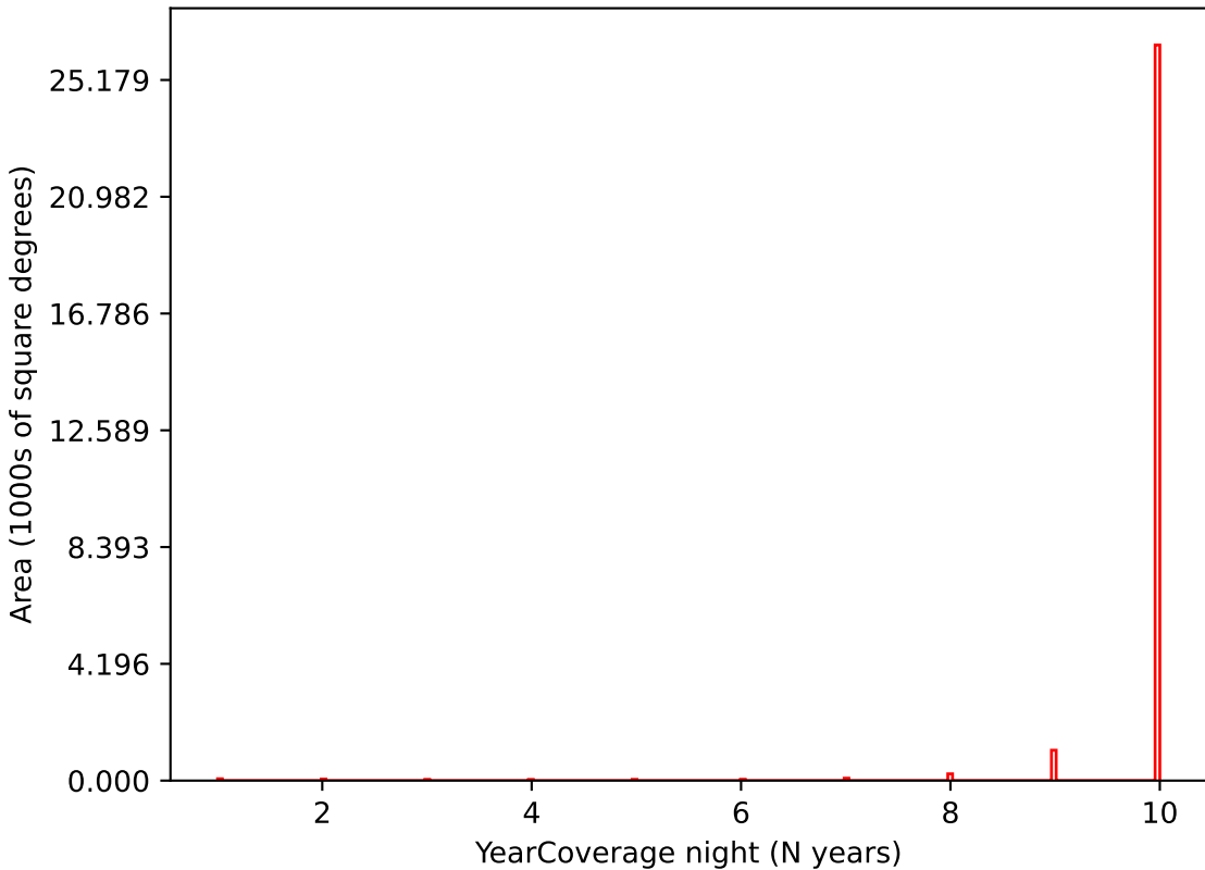
ddf_loaded_fl4_v3.4_10yrs i band: YearCoverage night
