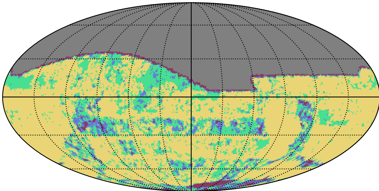
ddf_loaded_fl4_v3.4_10yrs g band: YearCoverage night
