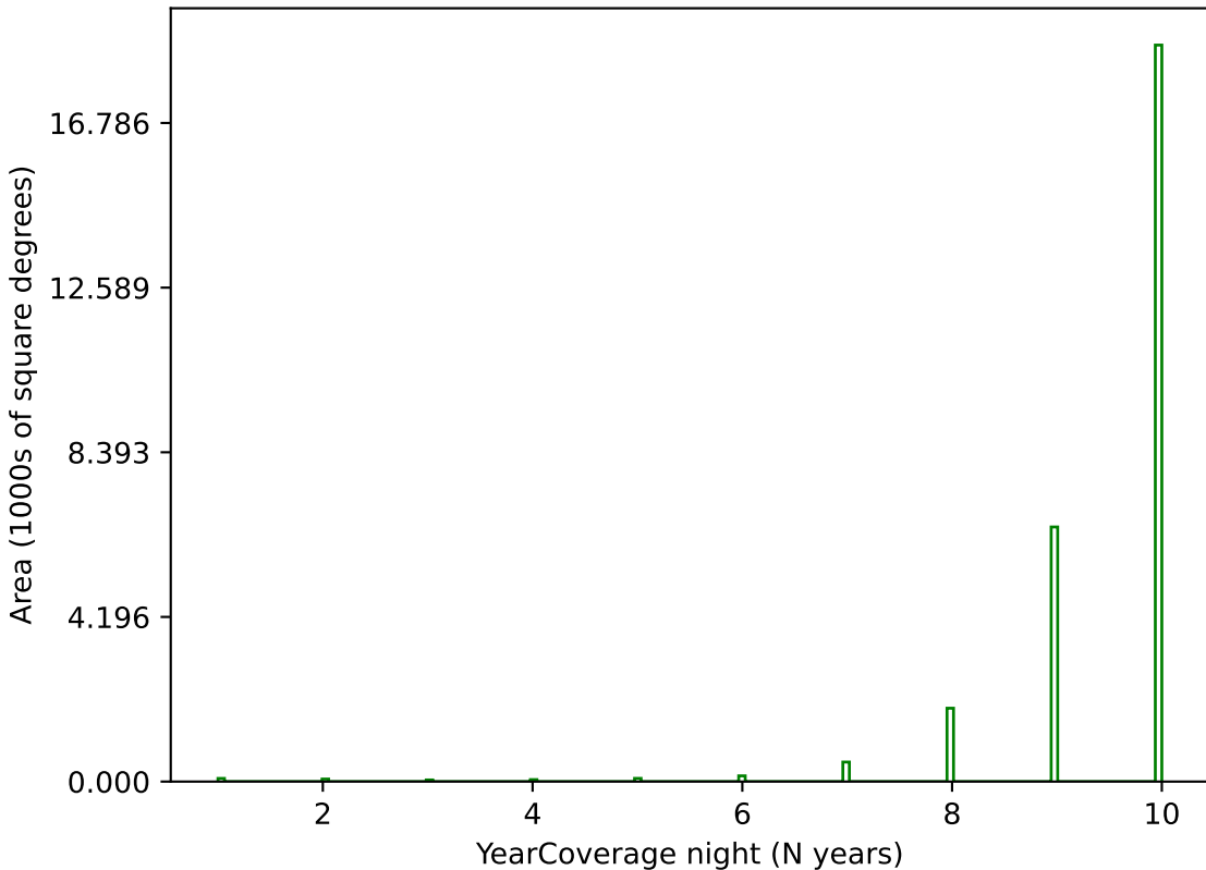
ddf_loaded_fl4_v3.4_10yrs g band: YearCoverage night
