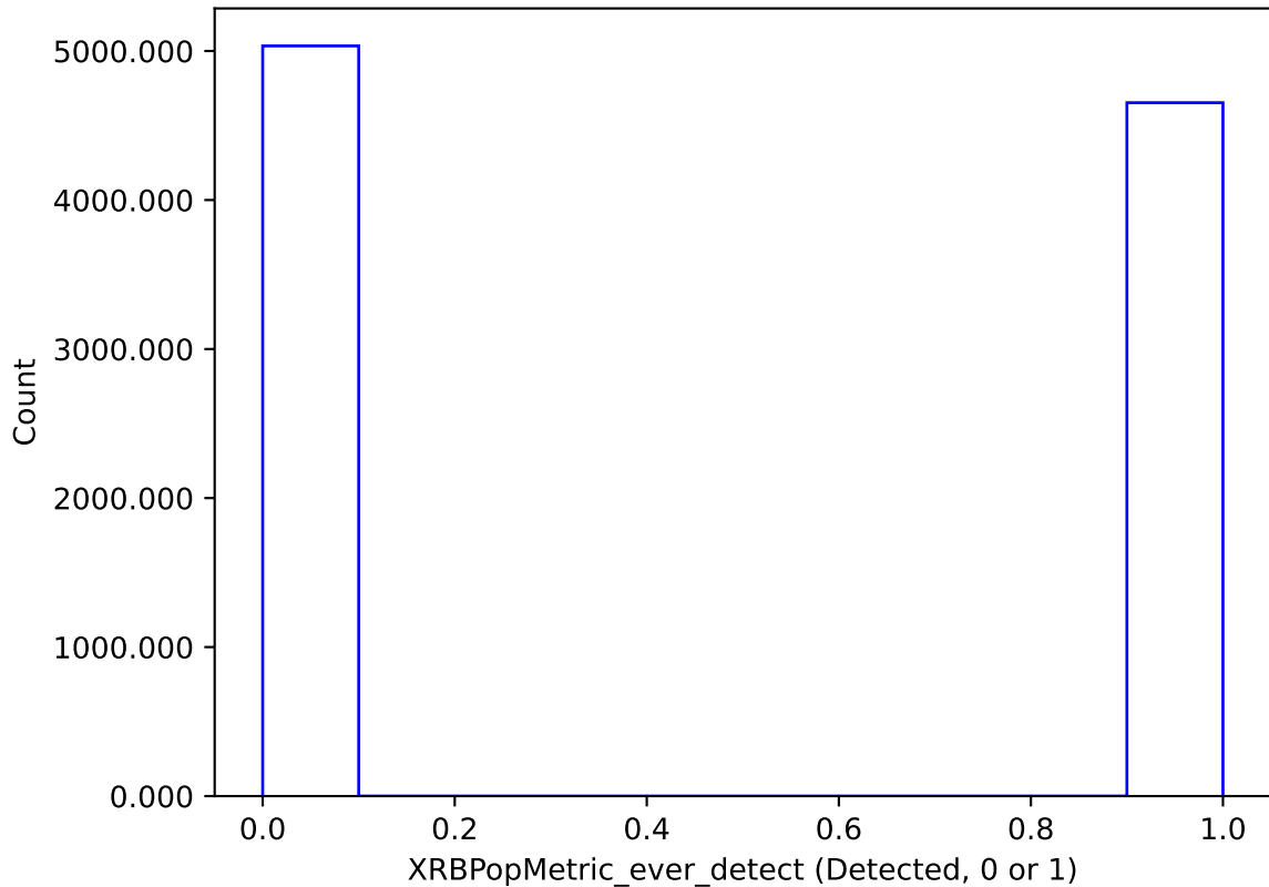
ddf_loaded_fl4_v3.4_10yrs : XRBPoMetric_ever_detect
