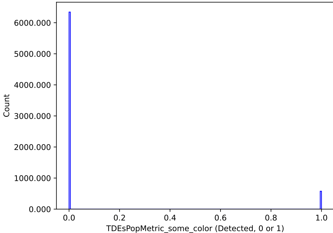
ddf_loaded_fl4_v3.4_10yrs : TDEsPopMetric_some_color
